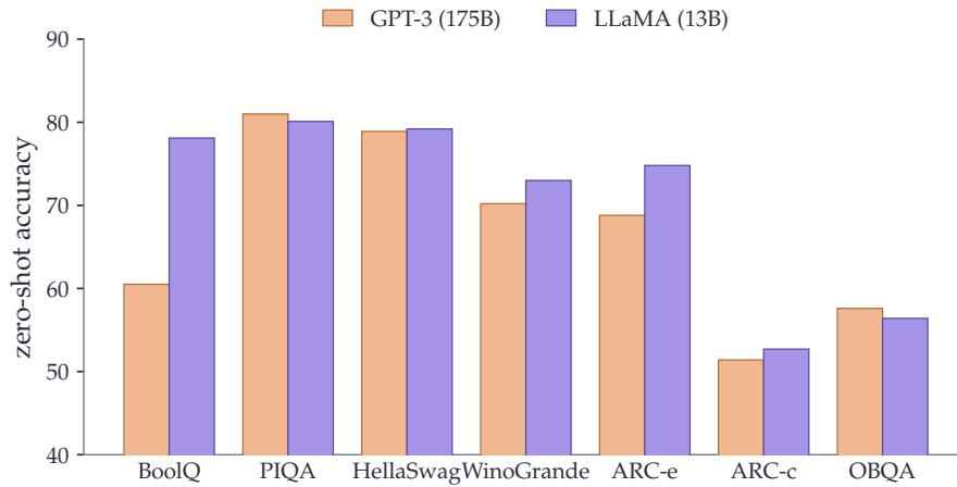
Figure 5.9: A 13-billion-parameter model trained on more tokens matches or beats GPT-3, which is more than ten times larger, on most of these zero-shot reasoning tasks. Numbers are verbatim from Table 4 of Touvron et al. (2023) .
