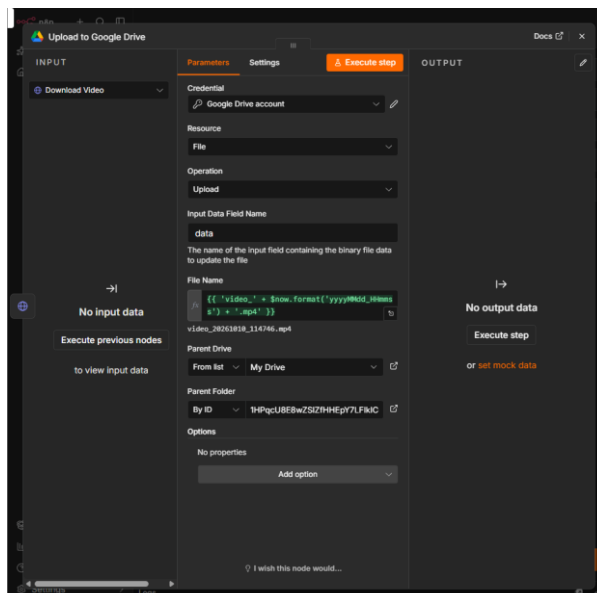
Gambar 9. Konfigurasi node Upload to Google Drive
