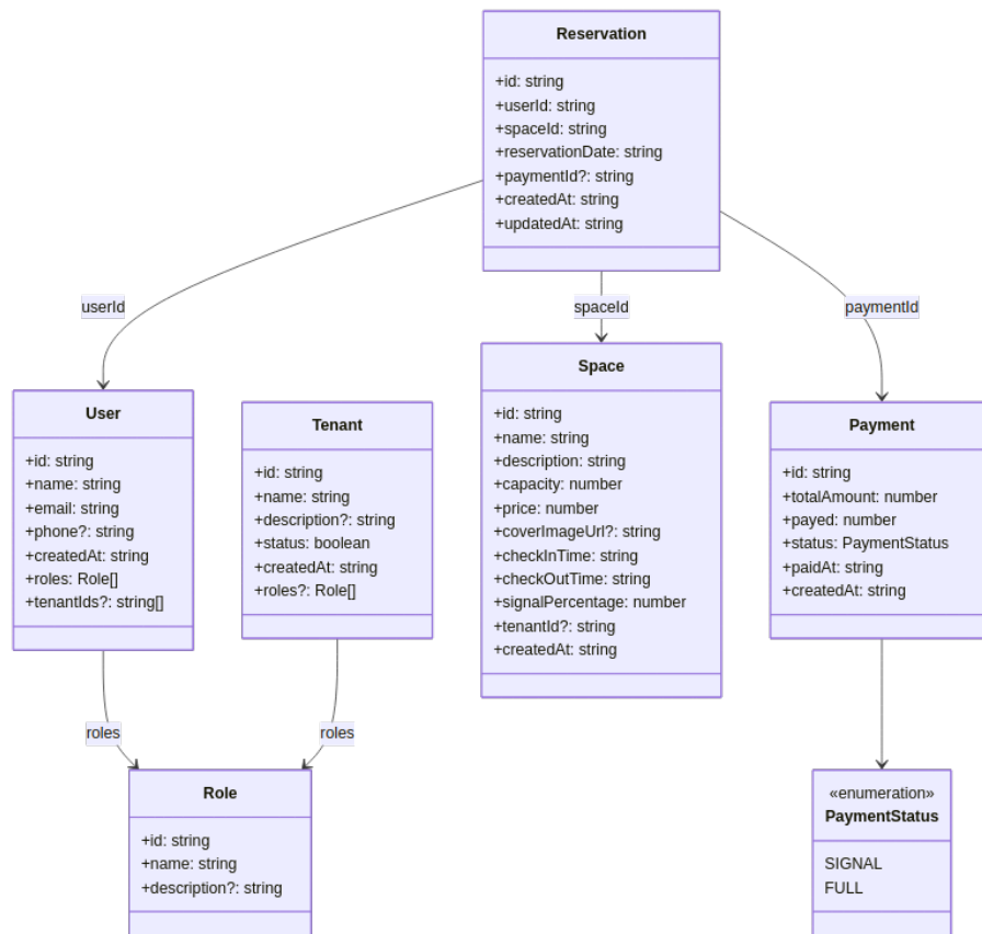
Figure 2: Diagrama de Classes
