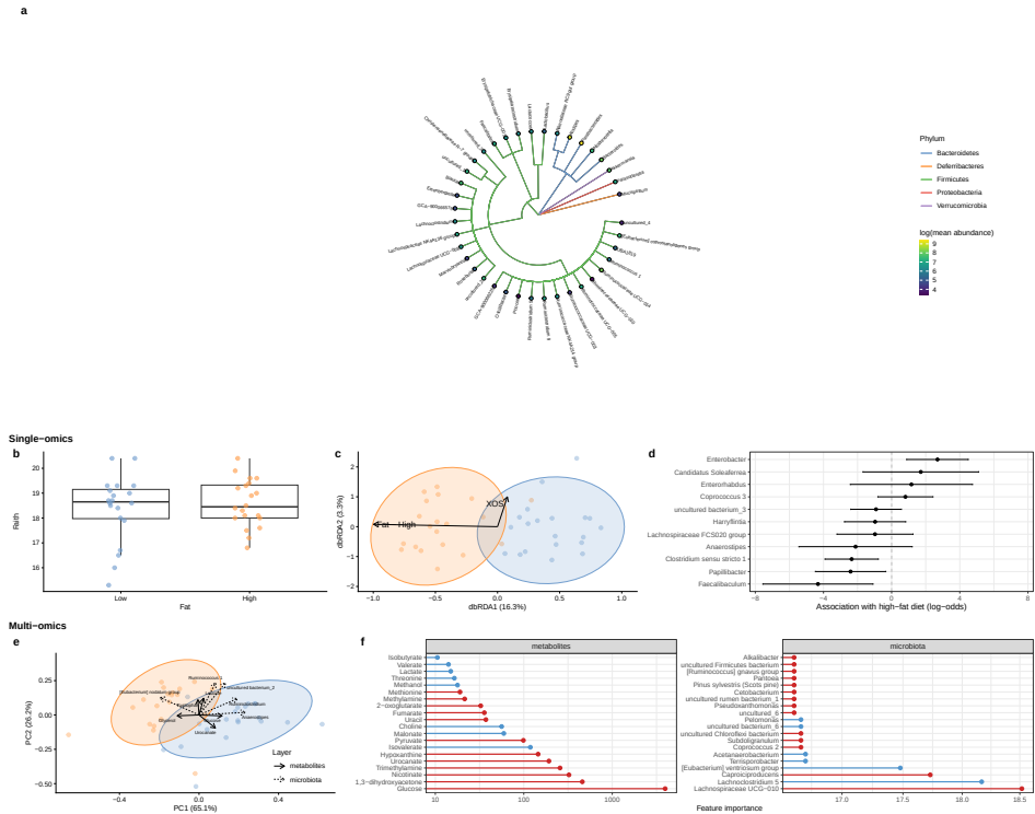
Figure 5: Selected single-omic and multi-omic visualizations for microbiome data. The figure demonstrates visualization workflows available in the ecosystem using the openly available multi-omics mouse dataset distributed through the mia package 85 . The dataset contains microbiota (16S rRNA) and metabolomics measurements from mice receiving either a high-fat or low-fat diet, with or without xylooligosaccharide (XOS) supplementation. a , Taxonomic relationships among bacterial genera represented as a tree. Most genera belong to the phylum Firmicutes , while Alistipes and Parabacteroides have the highest mean abundances. Single-omic analyses (b–d) demonstrate common analyses of individual microbiome data layers. b , Faith’s phylogenetic diversity 63 summarizes within-sample microbial diversity and shows no clear difference between diet groups. c , Distance-based redundancy analysis (dbRDA) based on UniFrac distances 66 visualizes differences in microbial community composition explained by the experimental variables, revealing separation according to diet. d , Differential prevalence analysis performed with MaAsLin3 71 identifies bacterial genera whose prevalence differs significantly between diet groups (adjusted P < 0.05 ). Multi-omic analyses (e–f) integrate microbiota and metabolomics data. e , Joint-RPCA provides an unsupervised low-dimensional representation of the combined microbiota and metabolomics data. The five strongest loading vectors from each data layer indicate the features contributing most to the displayed ordination axes. Vectors pointing in similar directions indicate positively associated features, whereas vectors pointing in opposite directions indicate negative associations. f , Signed feature importances from an IntegratedLearner model quantify the contribution of individual microbiota and metabolite features to supervised prediction of dietary group, indicating that metabolite features are generally more predictive than microbiota features, with glucose identified as the most important predictor.
