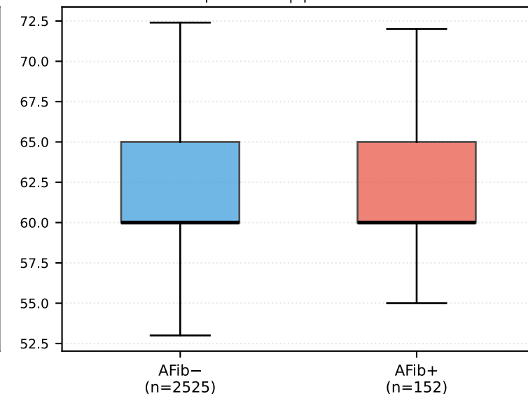
eGFR p = 0.049 | \beta = +0.1869
