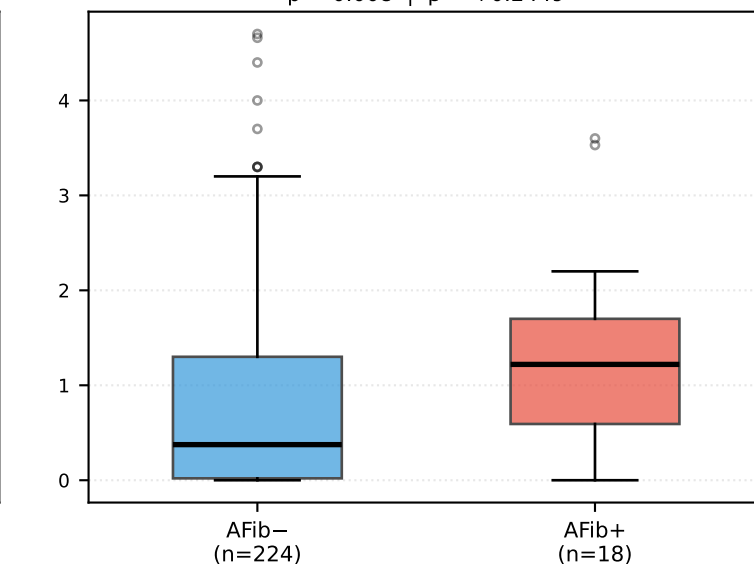
SVES p = 0.008 | \beta = +0.2449
