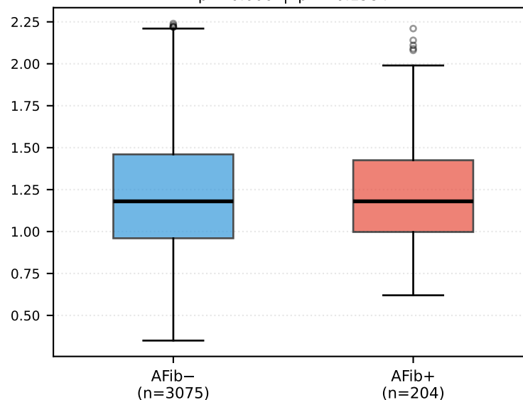
CHA 2 DS 2 -VASc p < 0.001 | \beta = +0.0580
