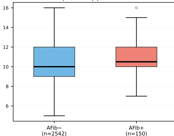
HDL p = 0.006 | \beta = -0.1984
