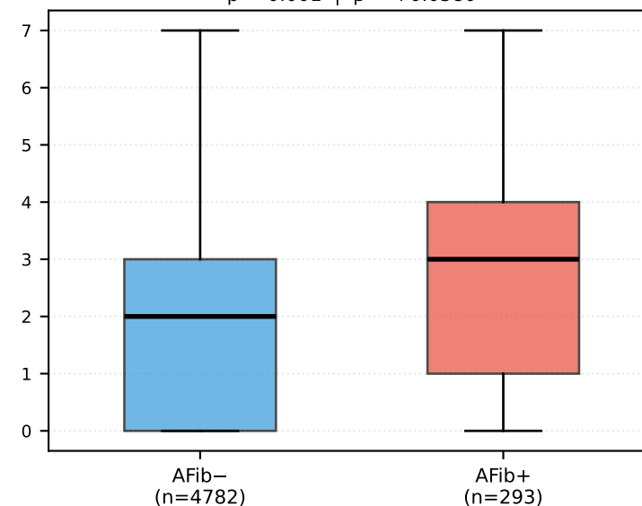
CHA 2 DS 2 -VASc p < 0.001 | \beta = +0.0580
