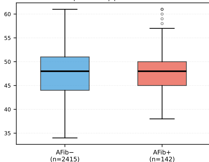
LDL p < 0.001 | \beta = -0.1522
