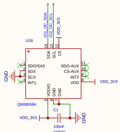
QMI8658A_I2C_ADD : 0x6a
