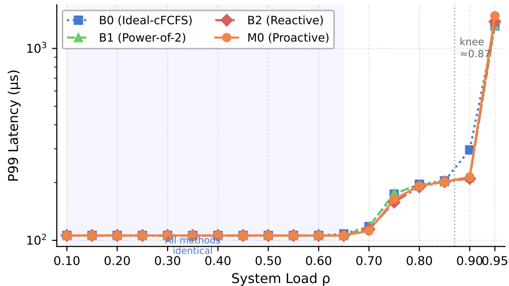
Fig. 1 W1 (Poisson+Bimodal): P99 vs. System Load Cluster: 64×16 cores, E[S]=24\ \mu\text{s} , 5 seeds median
