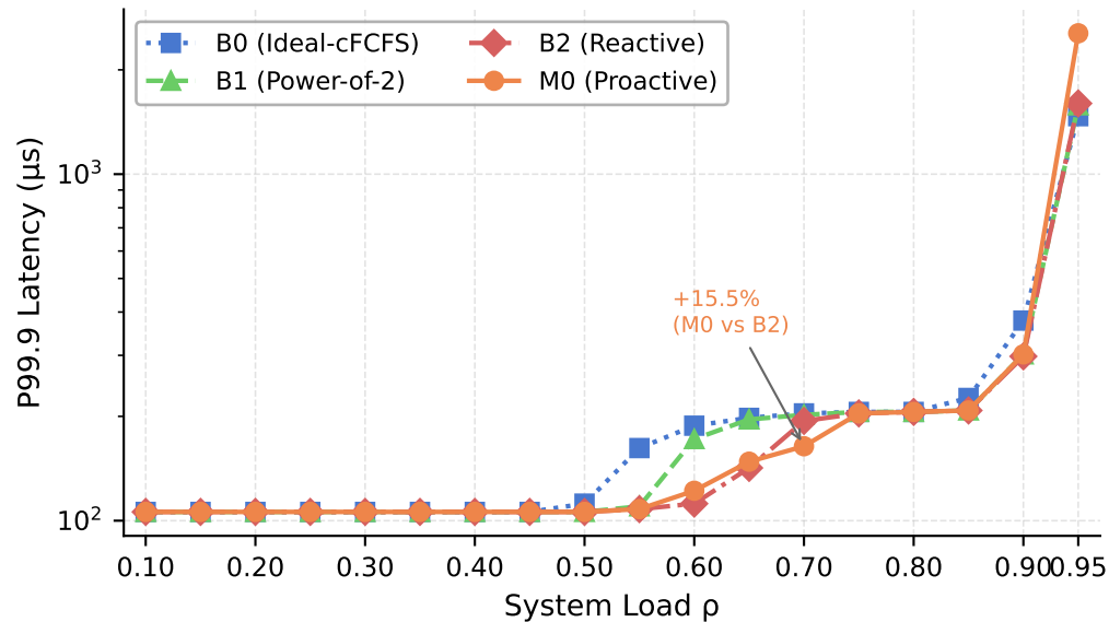
Fig. 2 W1 (Poisson+Bimodal): P99.9 vs. System Load 5 seeds median; M0 shows +15.5% P99.9 gain at \rho=0.70
