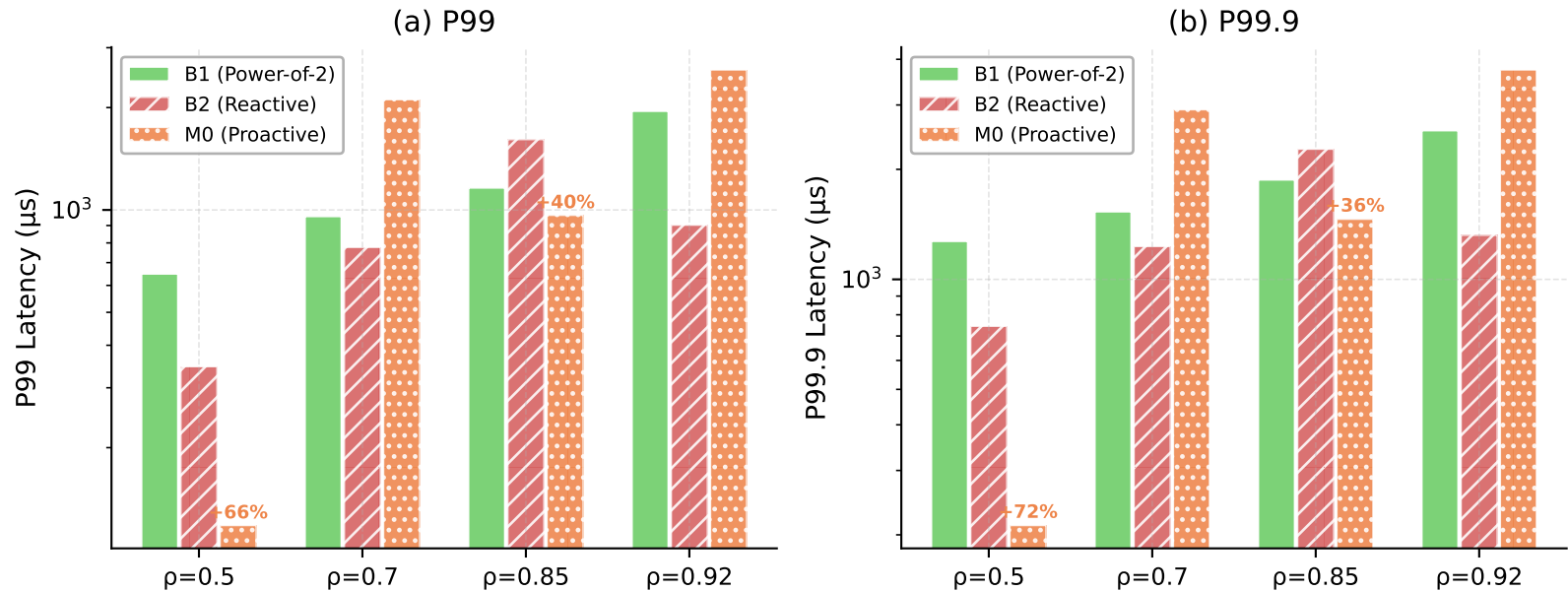
Fig. 3 W2 (MMPP+Bimodal) Burst Scenario: P99 and P99.9 Comparison M0 annotation shows improvement over B2 (5 seeds median)
