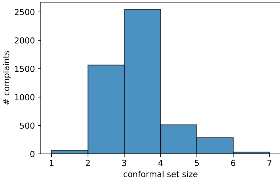
Conformal set sizes ( \alpha=0.1 , mean=2.90)
