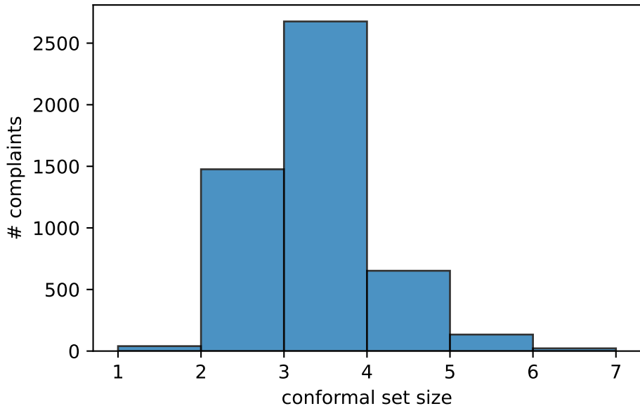
Conformal set sizes ( \alpha=0.1 , mean=2.89)
