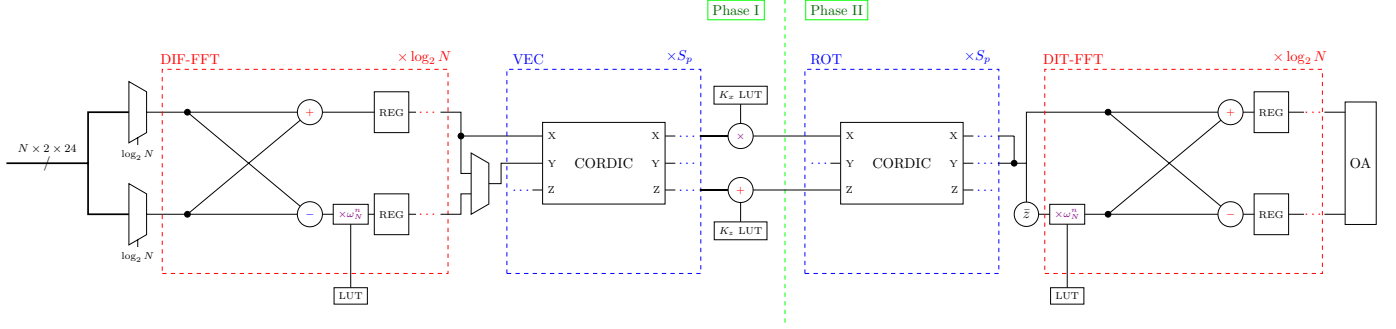
Fig. 5. Fully-pipelined FFT-conv design.
