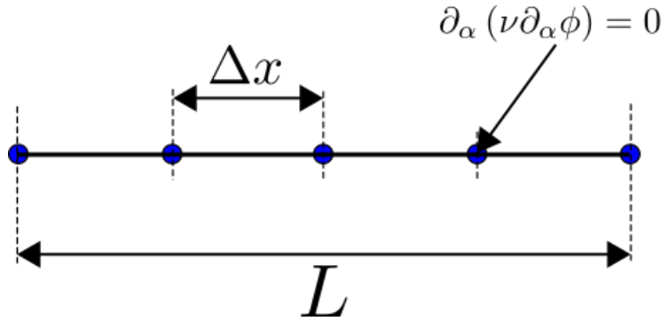
Fig. 2.1: 1D regular grid example for diffusive equation.
