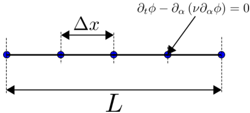
Fig. 1.1: 1D regular grid example for diffusive equation.
