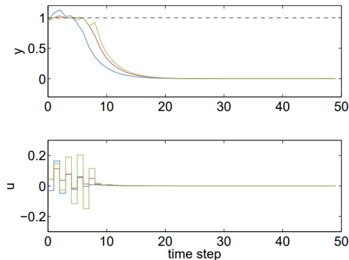
Figure 8.11: Soft constraints with combined quadratic and linear penalty for x(0) = \begin{bmatrix} 0.95 & 0.95 & 0.95 \end{bmatrix}^\top . A sufficiently large linear weight v promotes exact satisfaction of the constraint whenever this is possible.
