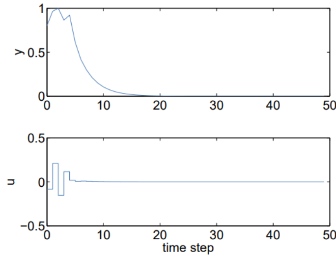
Figure 8.9: Third-order nonminimum-phase example used to illustrate soft constraints. The output constraint is -1 \leq y \leq 1 , with Q = C^\top C , R = 1 , and horizon N = 20 .
