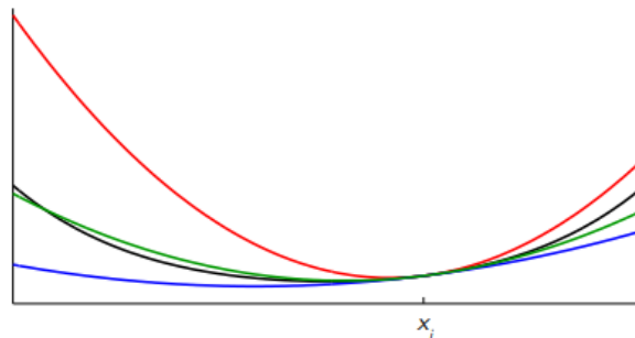
Figure 11.5: Newton's method. At the current iterate x^{(i)} , the function is approximated by a second-order Taylor model. The Newton step minimizes this local quadratic model. Unlike the L -smoothness upper bound, this quadratic approximation is not necessarily a global upper bound on f .
