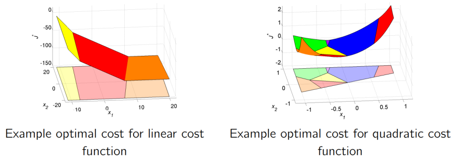
Figure 10.2: Piecewise structure of the nominal MPC value function. For linear MPC with polytopic constraints, a linear cost leads to a piecewise affine value function, while a quadratic cost leads to a piecewise quadratic value function. On compact feasible regions, such functions are Lipschitz continuous.
