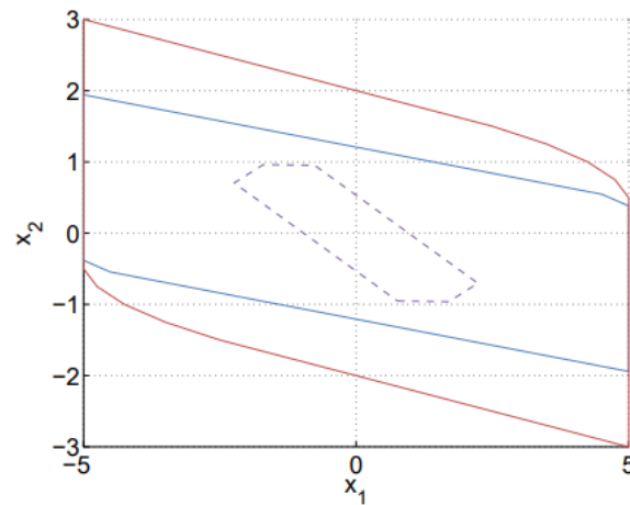
Figure 8.2: Comparison between the feasible set with and without terminal constraint. The blue line is the feasible set with terminal constraint. The red line is the feasible set without terminal constraint. The dashed line is the terminal set.
