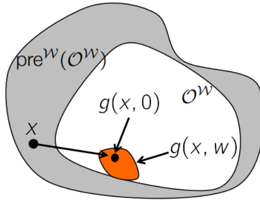
Figure 9.2: Geometric interpretation of the condition \mathcal{O}_{\mathcal{W}} \subseteq \text{pre}_{\mathcal{W}}(\mathcal{O}_{\mathcal{W}}) . The white region represents the set \mathcal{O}_{\mathcal{W}} , while the gray region represents its robust pre-set \text{pre}_{\mathcal{W}}(\mathcal{O}_{\mathcal{W}}) . For a state x to belong to the robust pre-set, all possible successors g(x, w) , for w \in \mathcal{W} , must remain inside \mathcal{O}_{\mathcal{W}} . The orange set illustrates the collection of possible successor states generated by the admissible disturbances. Since this whole set lies inside \mathcal{O}_{\mathcal{W}} , the point x belongs to \text{pre}_{\mathcal{W}}(\mathcal{O}_{\mathcal{W}}) .
