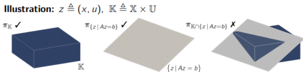
Figure 11.7: Implications of projected-gradient methods for MPC. With simple input constraints in a condensed formulation, projections may be cheap. With state constraints and dynamics, the feasible set becomes an intersection between simple constraint sets and the affine dynamics constraint, and projection onto the intersection is no longer straightforward.
