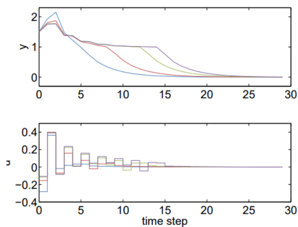
Figure 8.10: Soft constraints with quadratic penalty. Increasing S hardens the soft constraint: the size of the violation is reduced, but the duration of the violation can increase.
