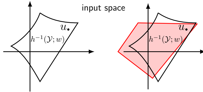
Figure 10: First-order approximation of the inverse image of the output constraint. Linearizing the steady-state map around the current input u transforms the nonlinear feasible set h^{-1}(\mathcal{Y}; w) into a local polyhedral approximation that is much easier to use in a projection step.
