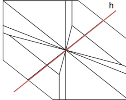
Figure 11.2: Offline construction of a search tree. A separating hyperplane is chosen so as to split the set of critical regions into two subsets of comparable size. The same construction is then repeated recursively on the two subsets.
