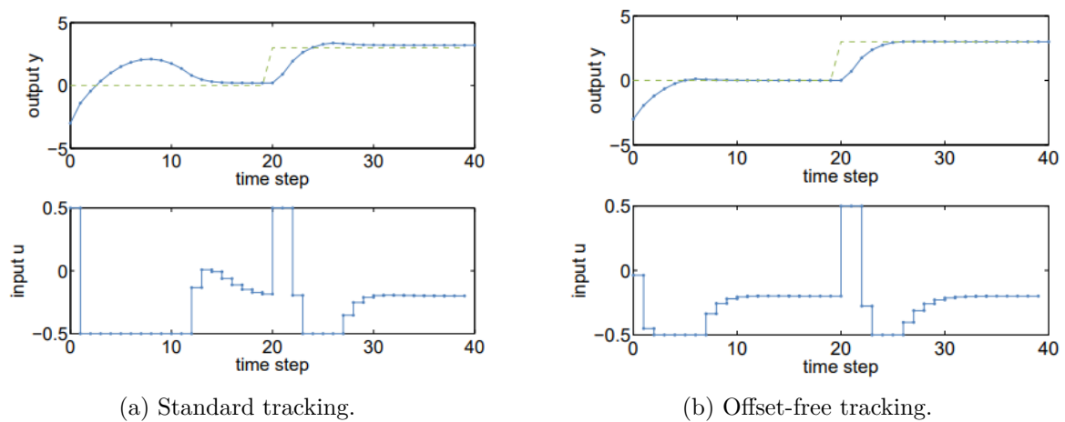
Figure 8.1: Comparison between standard tracking and offset-free tracking for the disturbed double integrator. Standard tracking stabilizes the system but exhibits a steady-state offset. Offset-free tracking estimates the constant disturbance and modifies the target condition, so that the output converges to the desired reference.
