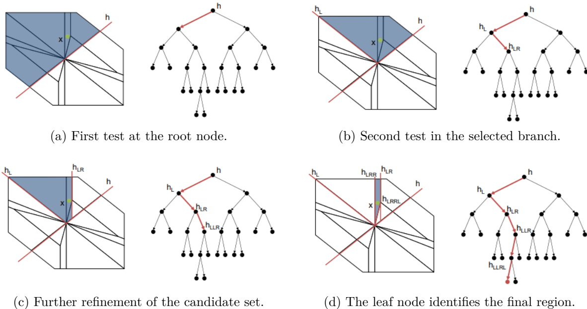
Figure 11.3: Logarithmic search for explicit MPC. The left part of each slide shows the progressive localization of the state in the polyhedral partition. The right part shows the corresponding path in the binary search tree. Each hyperplane test eliminates a large subset of candidate regions.
