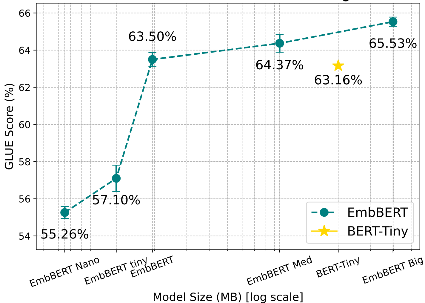
GLUE Score vs Model Size (semilog)
