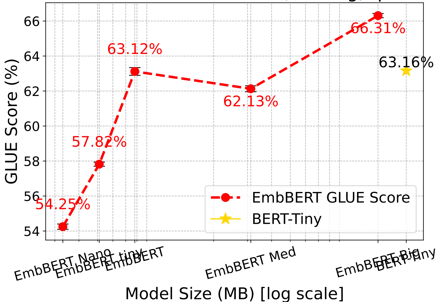
GLUE Score vs Model Size (semilog) quant
