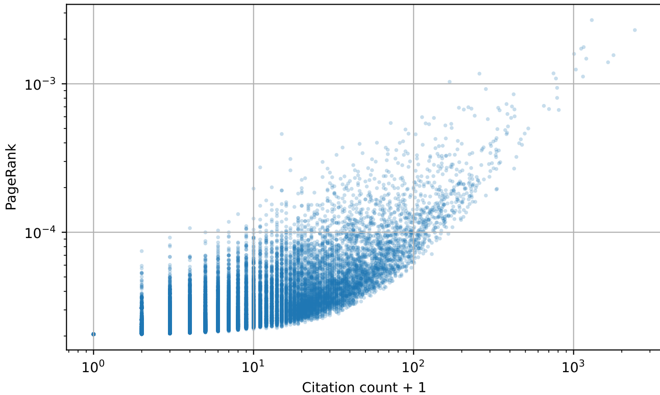
PageRank versus citation count
