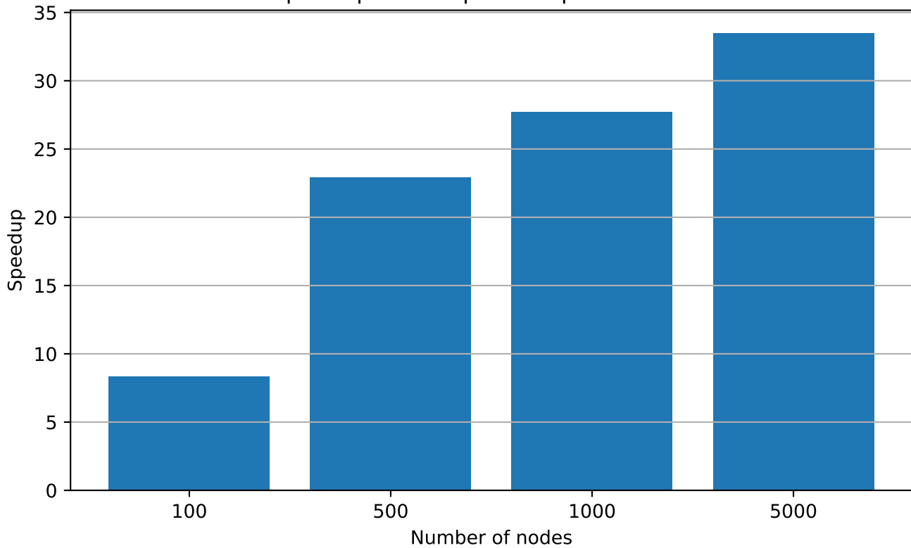
Speedup of the sparse implementation
