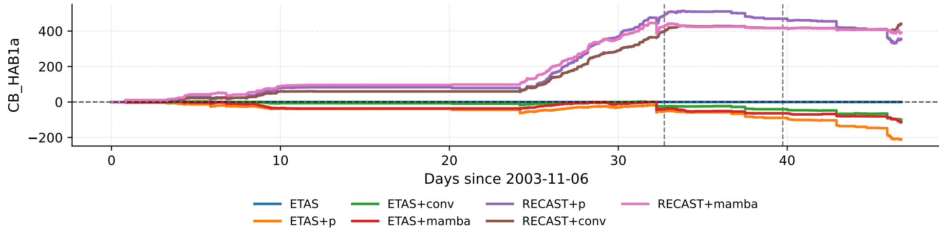
Cumulative Information Gain vs ETAS
