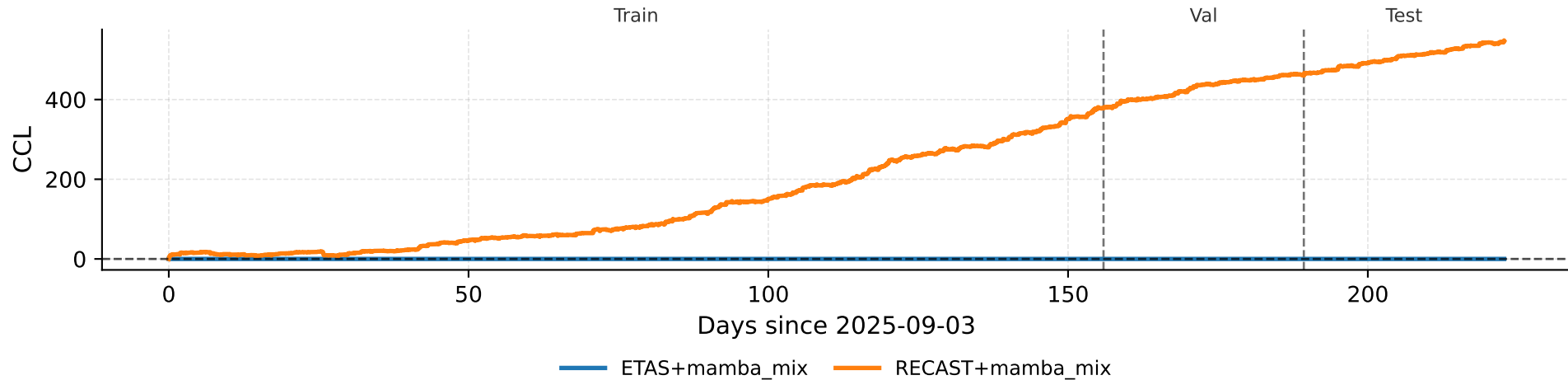
Cumulative Information Gain vs ETAS+mamba_mix
