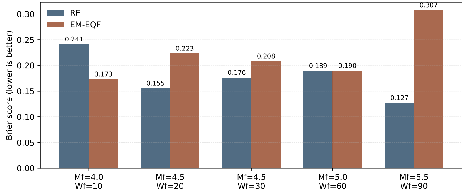
Brier Score Comparison (seed=0)
