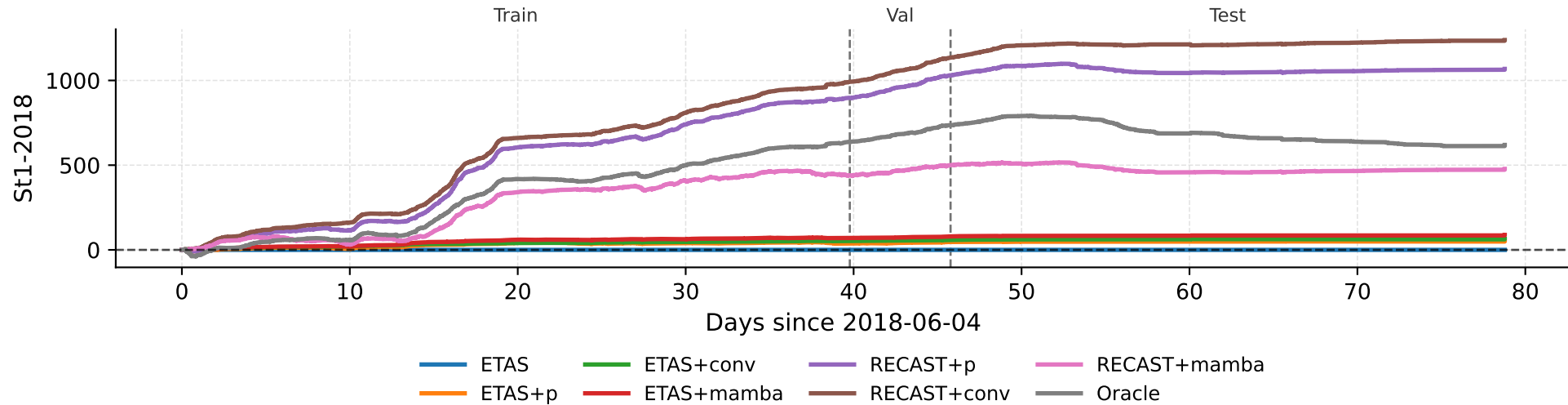
Cumulative Information Gain vs ETAS
