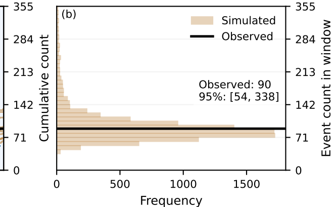
Forecast counts
