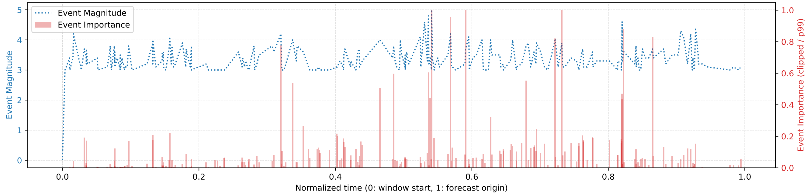
Event Magnitude and Event Importance (IG)
