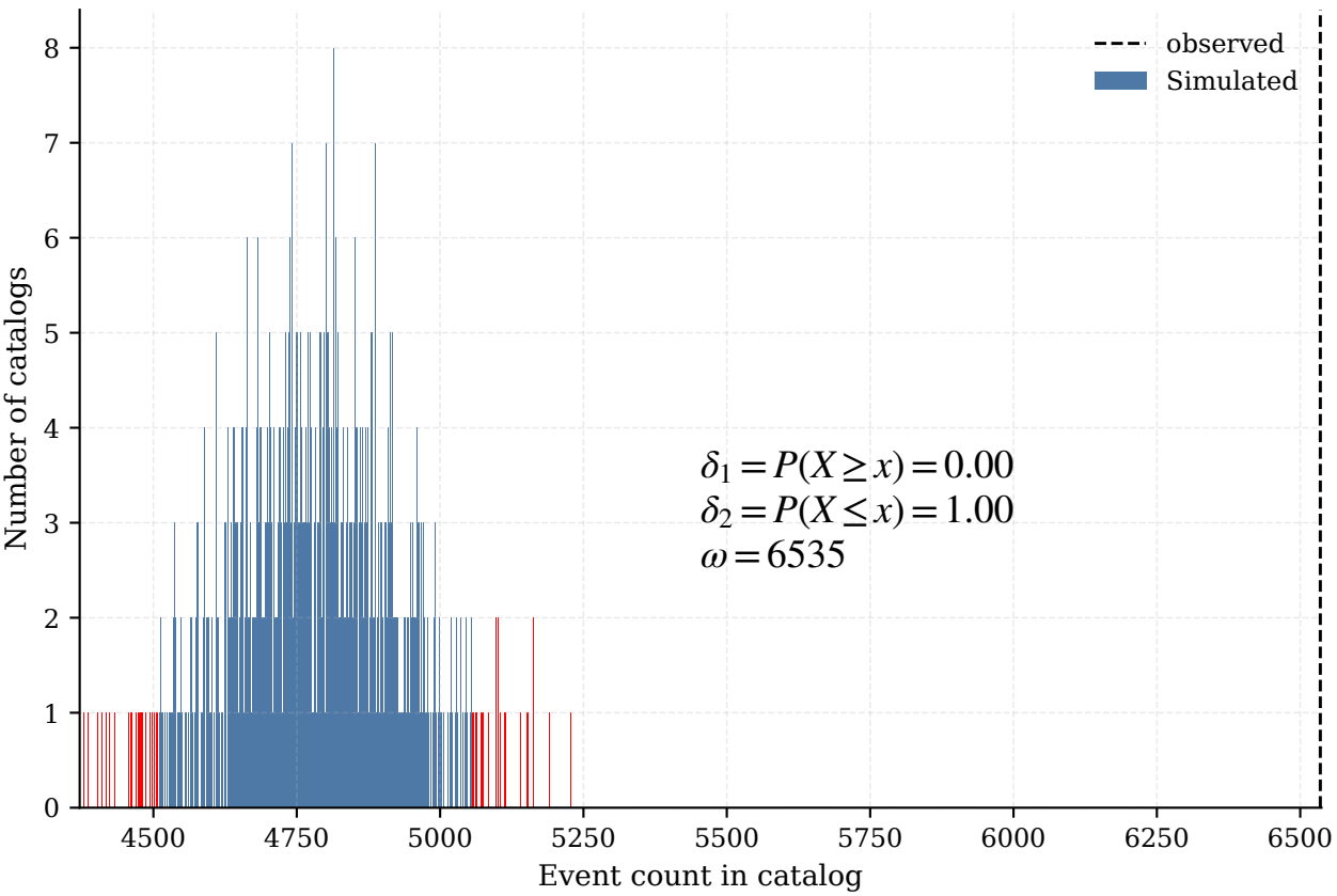
N-Test: Observed vs Simulated Event Counts
