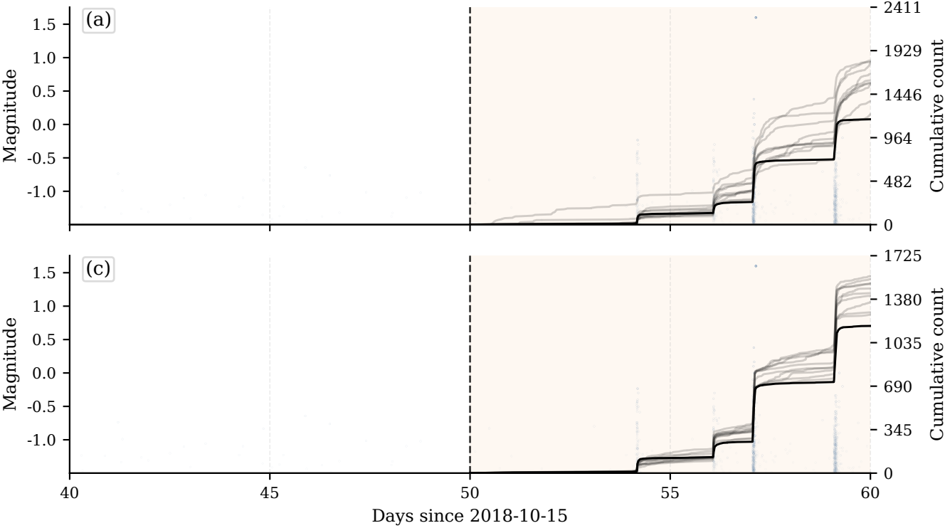
Observed Sequence and Example Forecast Trajectories
