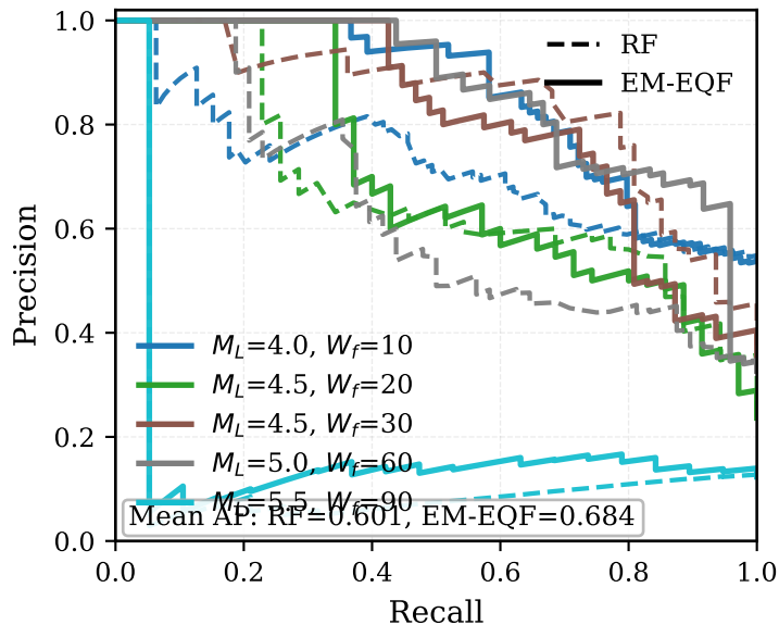
PR (All Windows)
