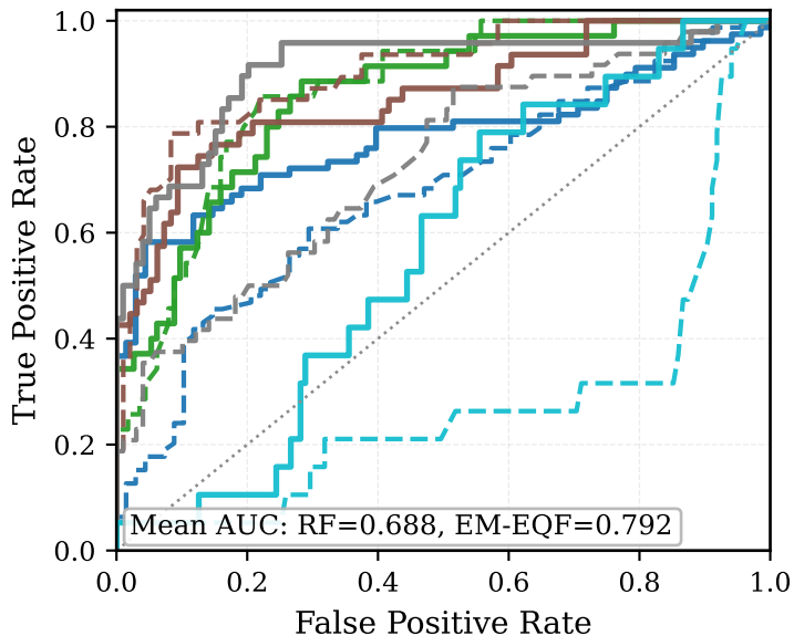
ROC (All Windows)
