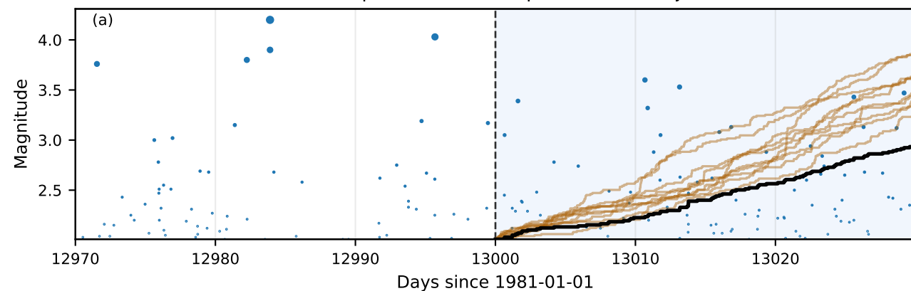
Observed Sequence and Example Forecast Trajectories
