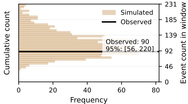
Forecast counts
