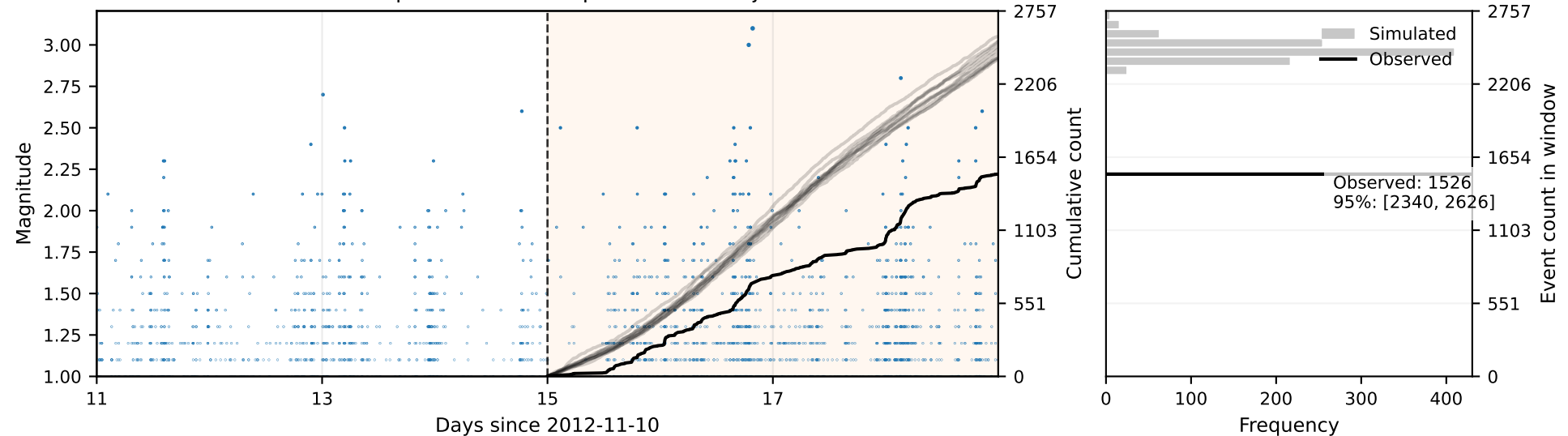
Observed Sequence and Example Forecast Trajectories
