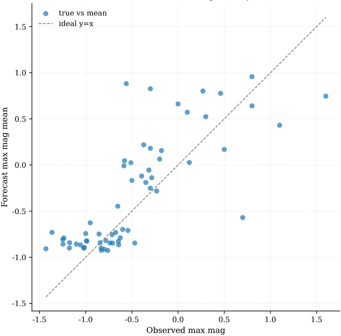
Observed vs Forecast Max Magnitude | MAE: 0.33
