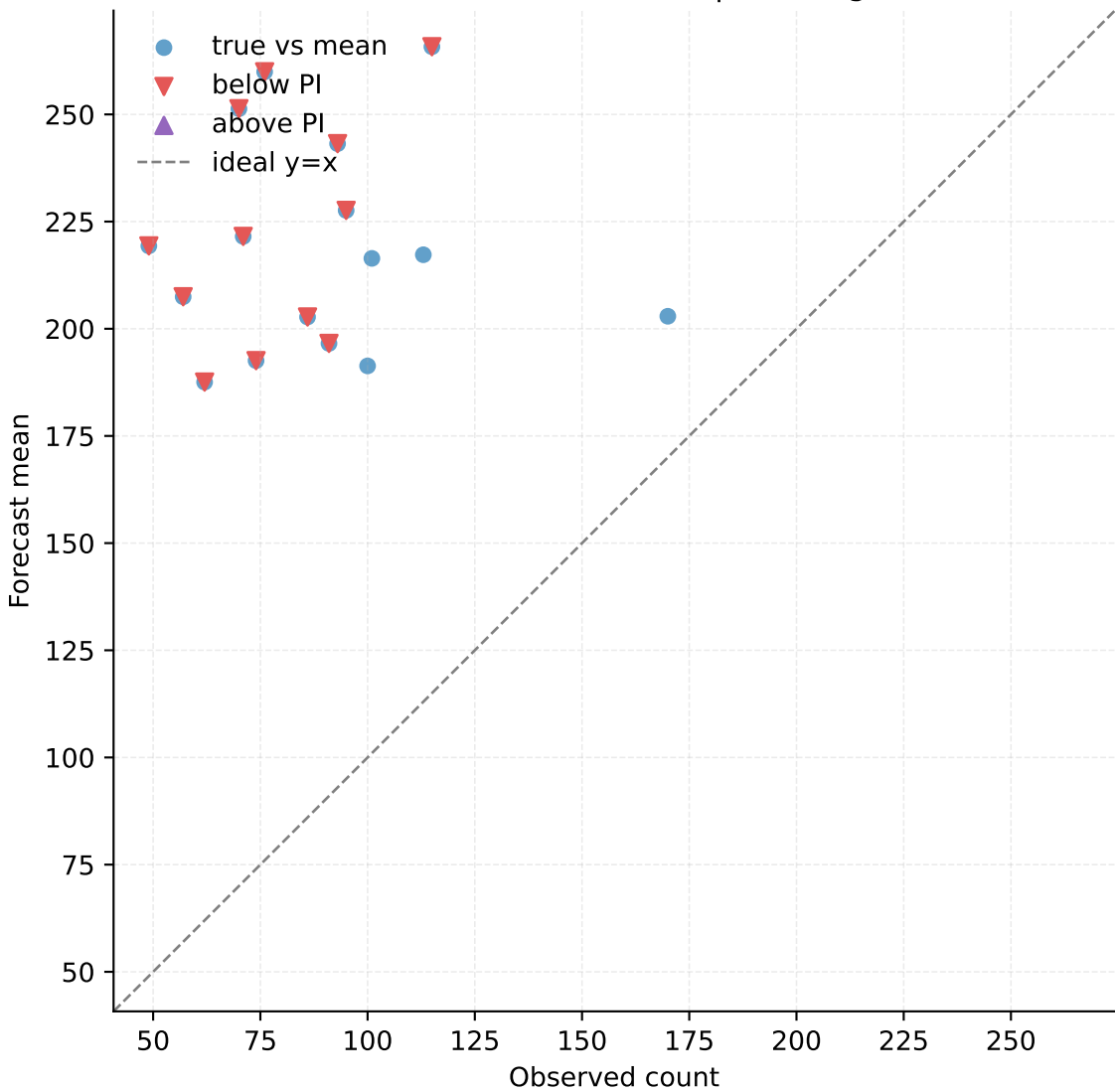
Observed vs Forecast (zoomed) | Coverage: 22.22%
