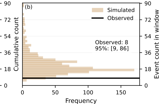
Forecast counts
