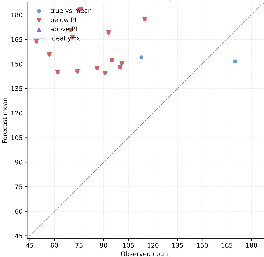
Observed vs Forecast (zoomed) | Coverage: 11.11%
