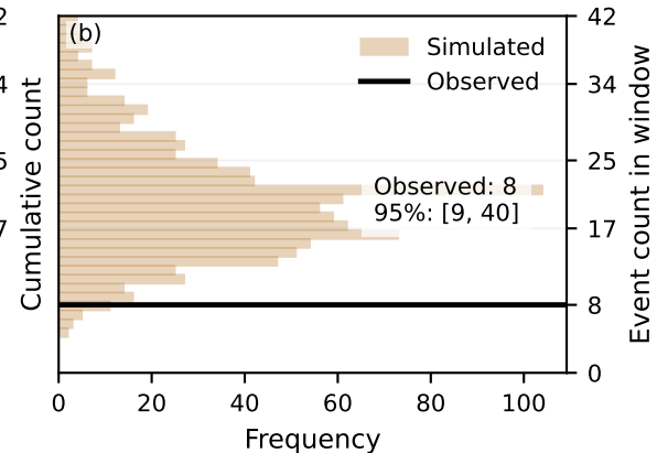
Forecast counts
