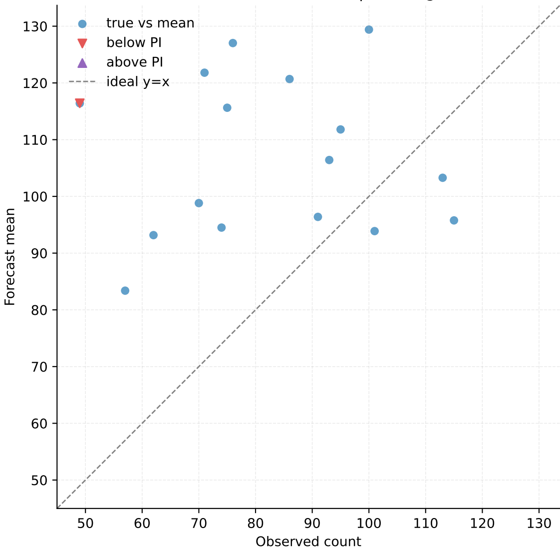
Observed vs Forecast (zoomed) | Coverage: 88.89%
