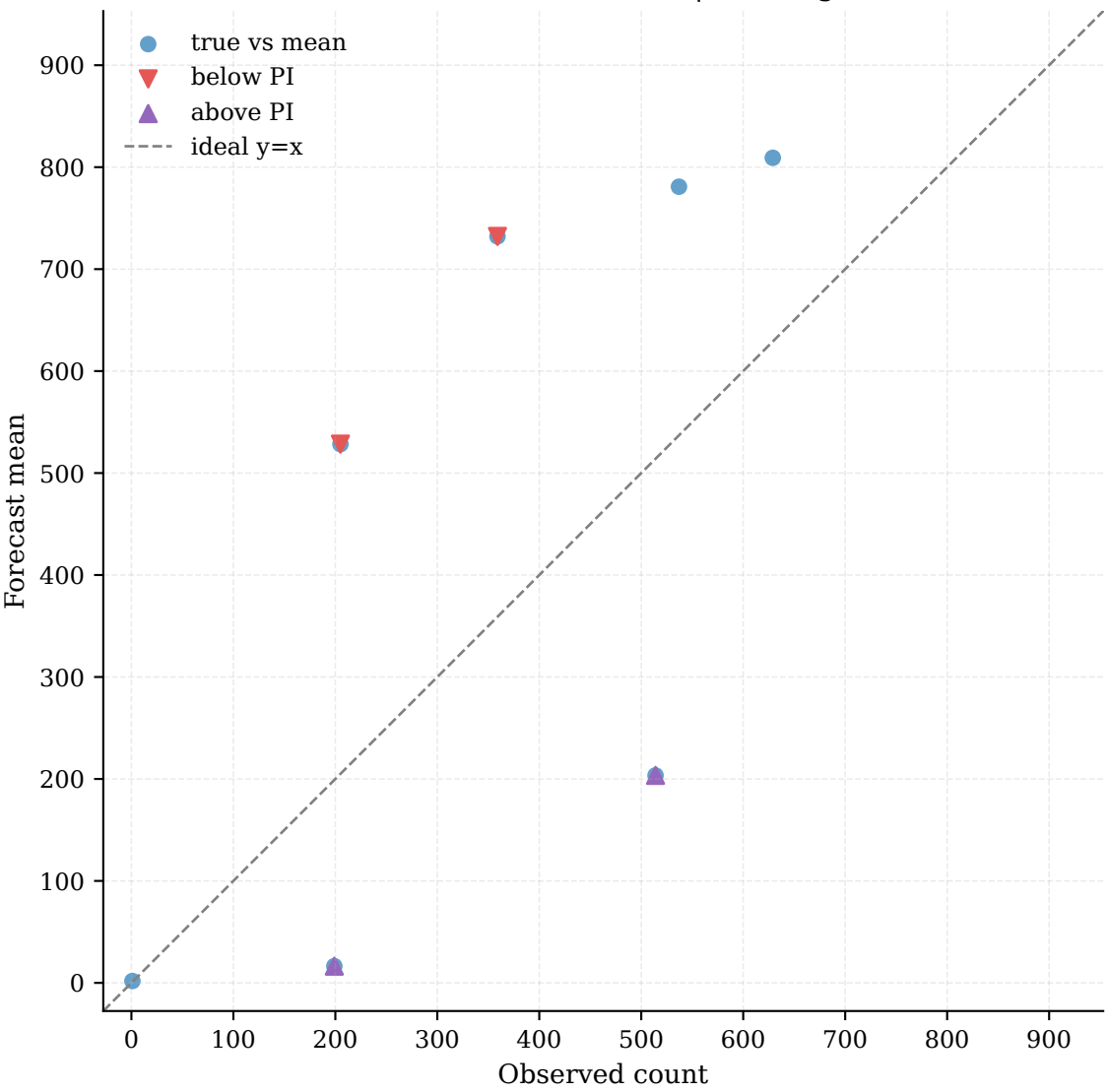
Observed vs Forecast (zoomed) | Coverage: 55.56%
