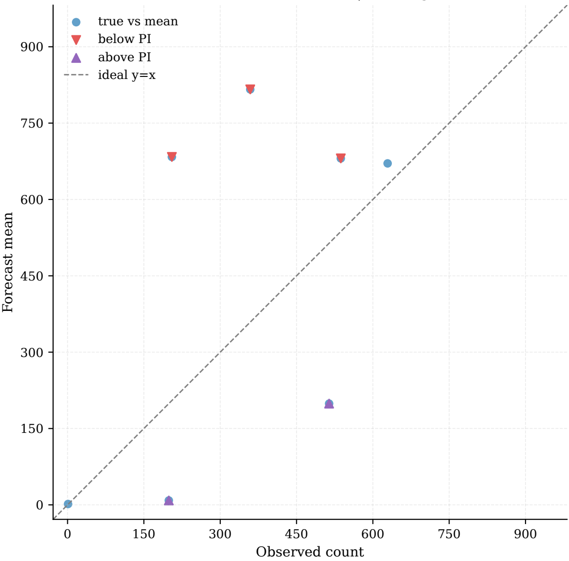
Observed vs Forecast (zoomed) | Coverage: 33.33%
