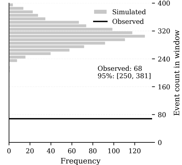
Forecast counts
