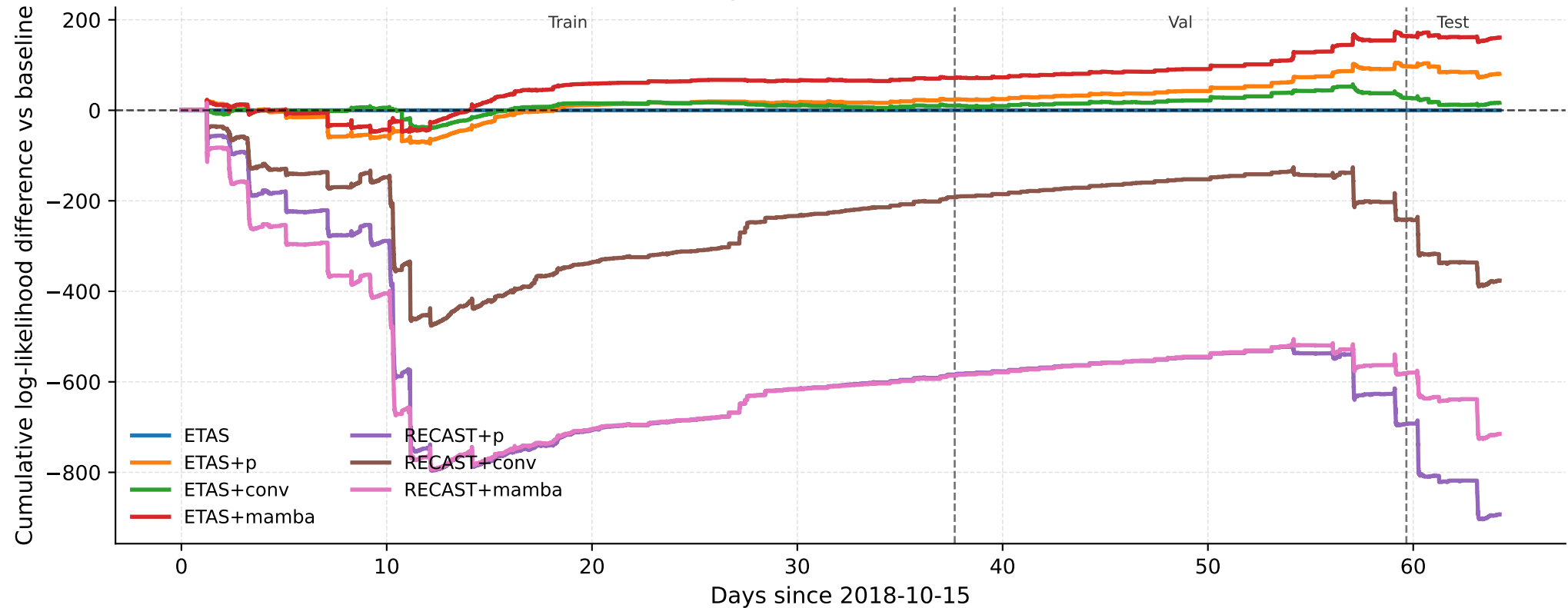
Cumulative log-likelihood difference over time
