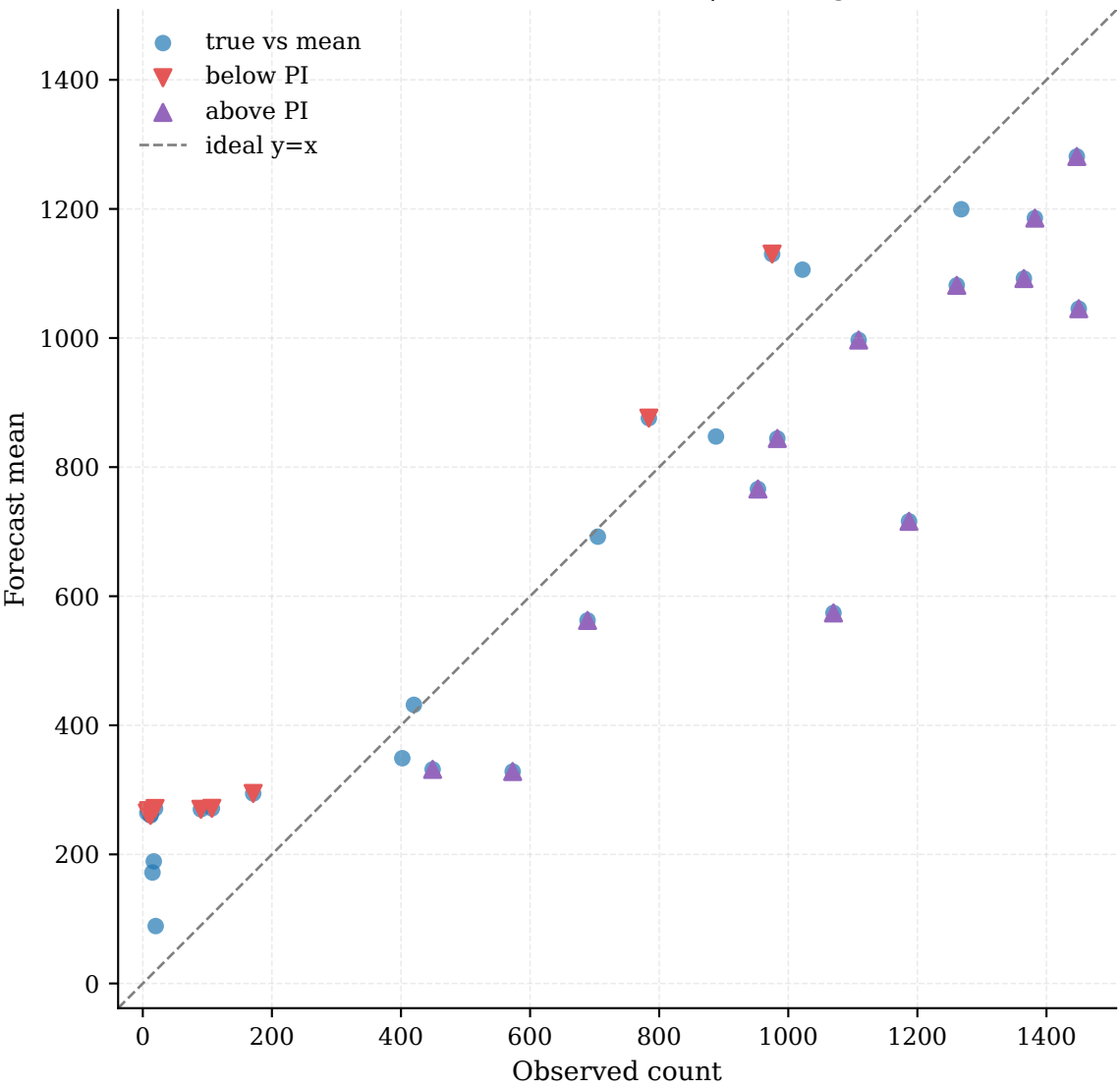
Observed vs Forecast (zoomed) | Coverage: 27.78%
