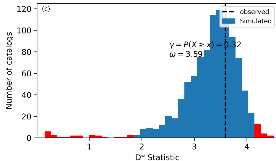
M-Test
