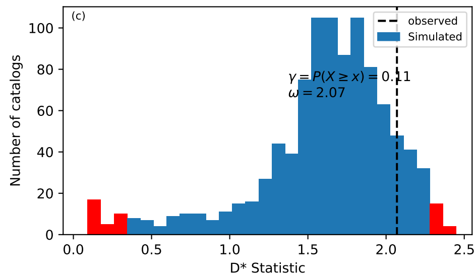
M-Test
