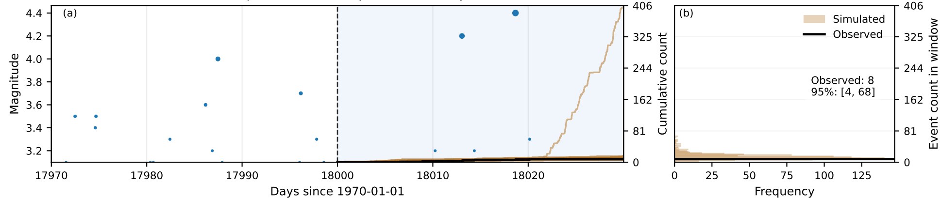
Observed Sequence and Example Forecast Trajectories
