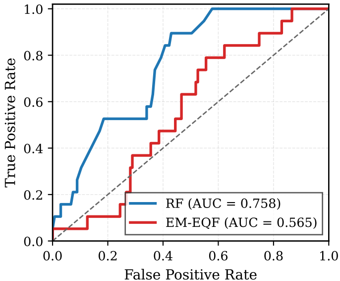
ROC Curve
