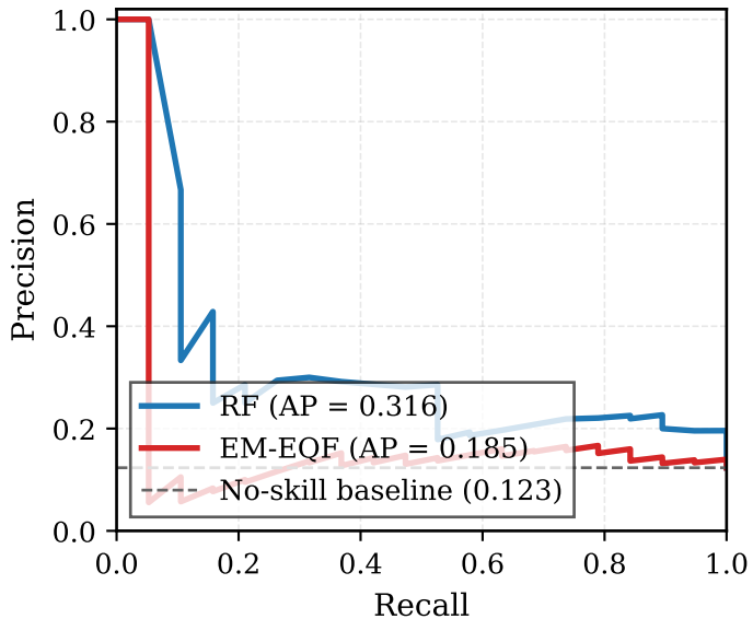
Precision-Recall Curve
