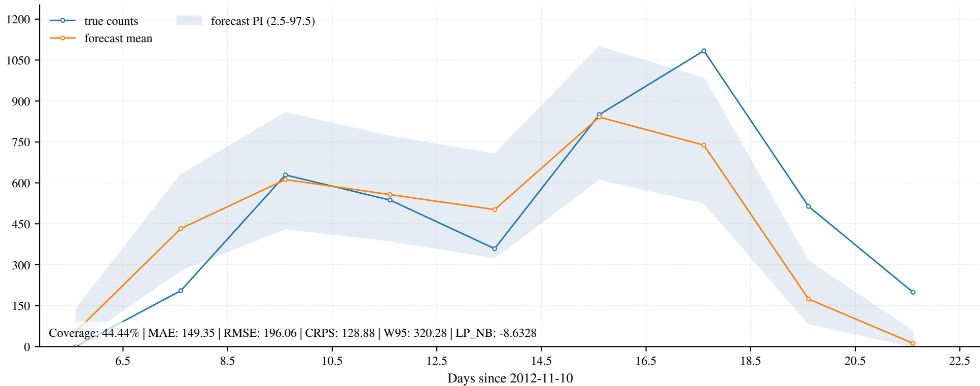
Counts: true vs forecast (zoomed)
