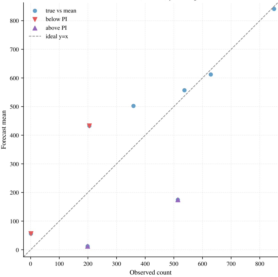
Observed vs Forecast (zoomed) | Coverage: 44.44%
